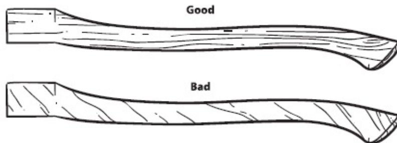
The grain of axe handles should run parallel to the wedge slot.
